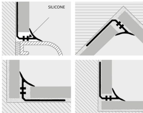
INTERNAL, EXTERNAL, THREE-WAYS PROINTER CORNER JOINTS ANODIZED GOLD (AO) or SILVER ALUMINIUM (AA) - pack. 2 Pcs
