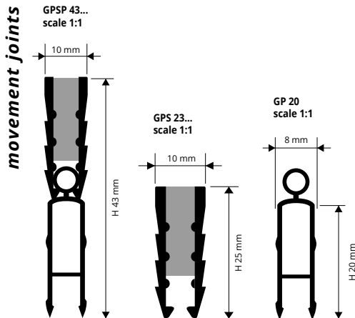
CO-EXTRUDED VINYL RESIN (PVC) WITH FULL SILICONE bar length 2,5 lm - pack. 40 Pcs - 100 lm
